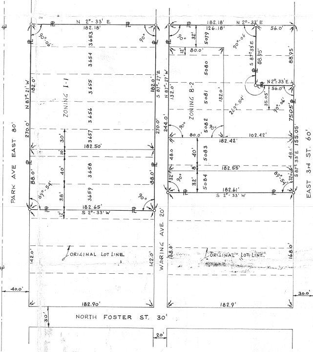
LOCATION PLAT SCALE: 1" = 50'
