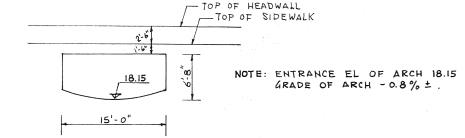
DETAIL OF BRICK & CONC ARCH FOR RITTER'S RUN ON EAST 3RD ST.
